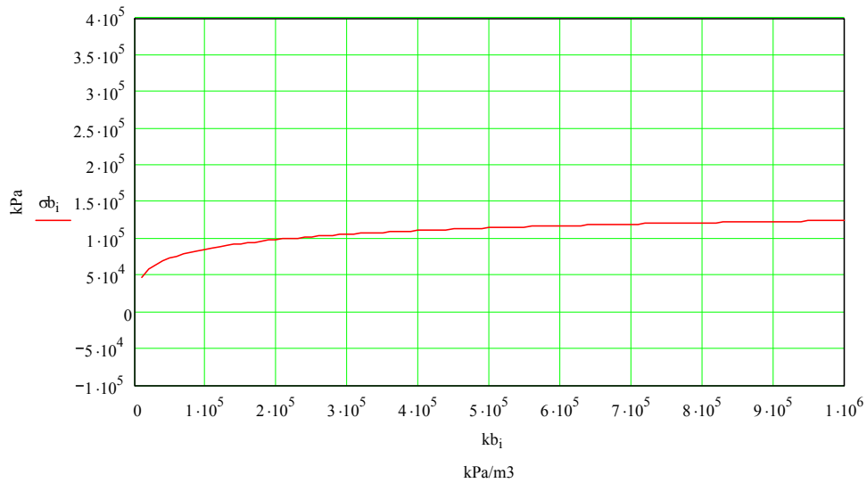
fig. 6 The stress variation in the annular bottom plates \sigma_b in the spot of joint between shell and bottom by meridional compression in joint -5 \text{ kN/m'} (tension)
