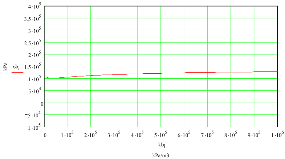
fig. 7 The stress variation in the annular bottom plates \sigma_b in the spot of joint between shell and bottom by meridional compression in joint -10 \text{ kN/m'} (tension)
