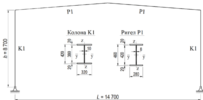
Fig. 1. Geometry and static scheme of typical steel frame, part of building in the town of Belovo.
