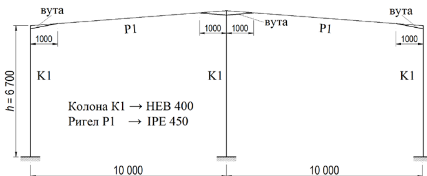
Fig. 2. Geometry and static scheme of typical steel frame, part of the building in the town of Kavarna
